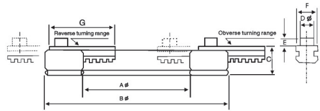
反轉位置：reverse turning range 正轉位置：obverse turning range
